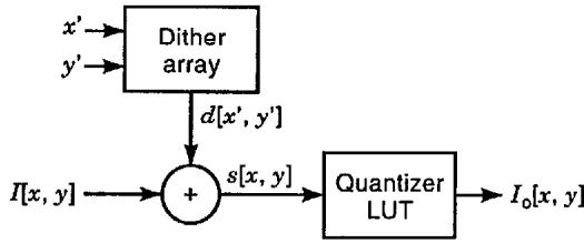
Figure 26. Dithering system with 2 LUTs.
