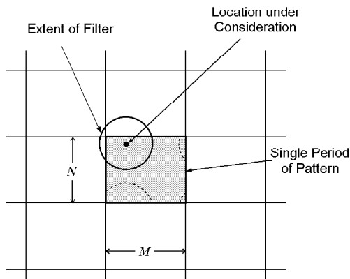
Figure 20. Two-dimensional periodicity of ordered dither pattern, and wraparound property of void-and-cluster-finding filters.
