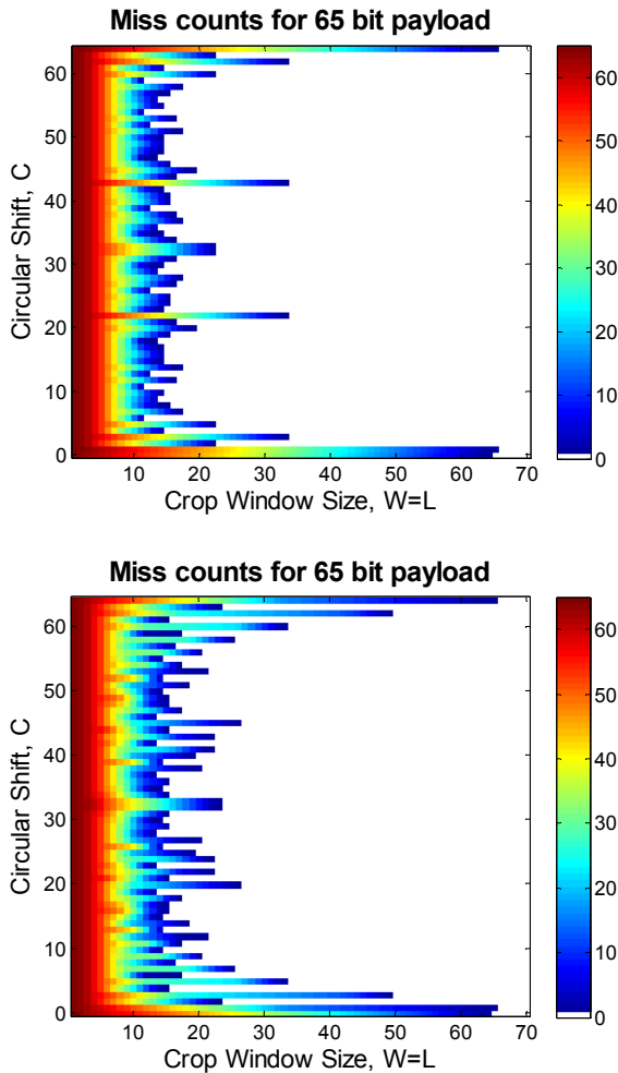
Figure 10. Worst case missed bits as function of crop window ( W=L ) and phase, C . Example where the number of payload bits is odd, B=65 . Results for an all highlight or all shadow region (top), and half highlight, half shadow region (bottom).
