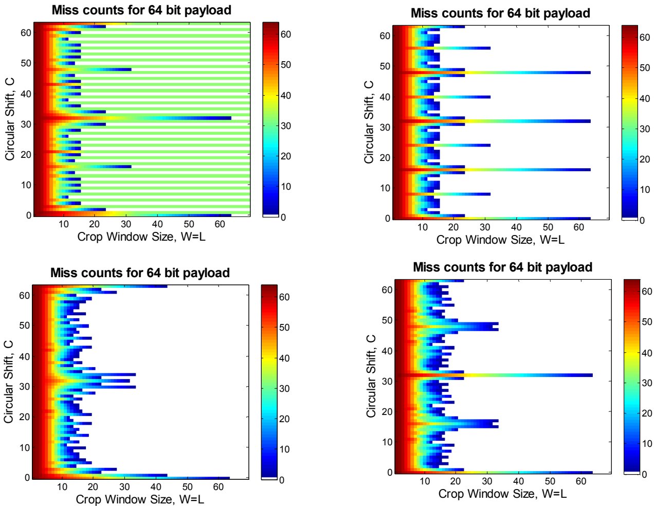
Figure 9. Worst case missed bits as function of crop window and circular shift. The B=64 example of Figure 8 for a payload with an even number of bits, but forcing the offset to be even by setting k=2 so D=2C . Results for an all highlight or all shadow region (top), and half highlight, half shadow region (bottom).
