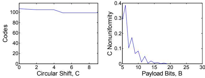
Figure 7. Uniformity testing of Circular Shifts C . Distribution for B=10 (left), and Relative Non-uniformity as a function of B (right).
