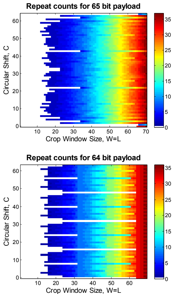
Figure 11. The 90% repeat counts for each bit in the payload as function of crop window and circular shift. The values indicate that 90% of the bits will be repeated at least that number of times. Results are shown for an all highlight or all shadow region. B=65, k=1 (top), B=64, k=2 (bottom).
